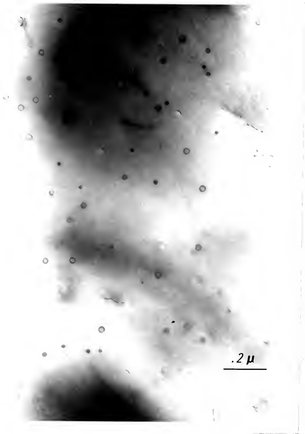
Figure 35.--Isolated colony of voids in a foil that was annealed for 100 hours at 500°C. Average void diameter is 300 Å.
